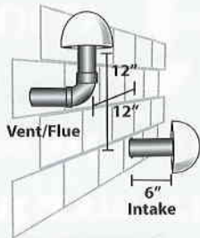
Horizontal Termination (Dual Pipe)
